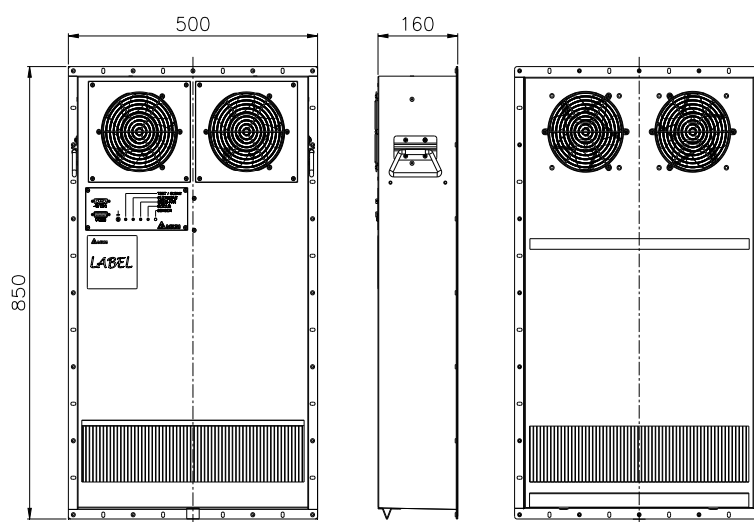
Dimension drawing
