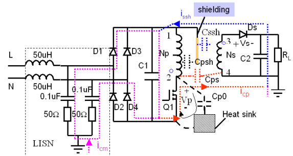
Fig.1. Coupling path of CM noise in Fly-back converter
