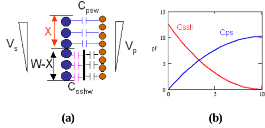
Fig.9. (a) Position of the open area of shielding at high voltage side winding; (b) effect of modulating shielding width
