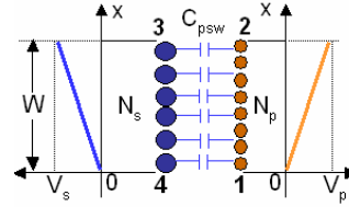
Fig.5. Voltage distribution and capacitive coupling in the open area
