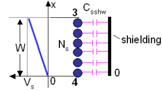
Fig.6. Voltage distribution and Capacitive coupling between Secondary winding and shielding
