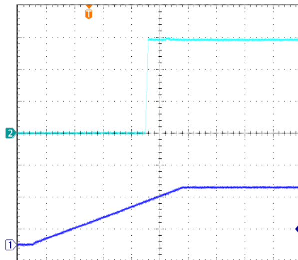
Figure 6: Input Voltage Start-up at full load
